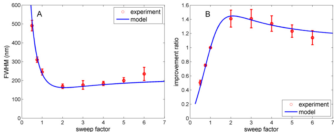
Fig. 4. Measured FWHM (A) and FWHM improvement ratio w.r.t. M = 1 (B) as a function of sweep factor M obtained from measurements on 9 beads, and the prediction of Eq. (1) with excitation and emission spot widths W_{ex} = 224 \text{ nm} and W_{em} = 235 \text{ nm} , showing a good agreement between the experiment and the model and a clear optimum in resolution improvement close to M = 2 .
